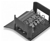
Fig. 6 - Typical Blower Resistor
